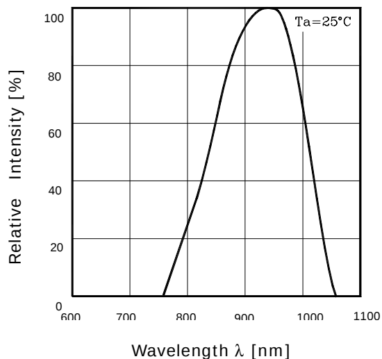
Fig. 5 Spectrum Sensitivity
