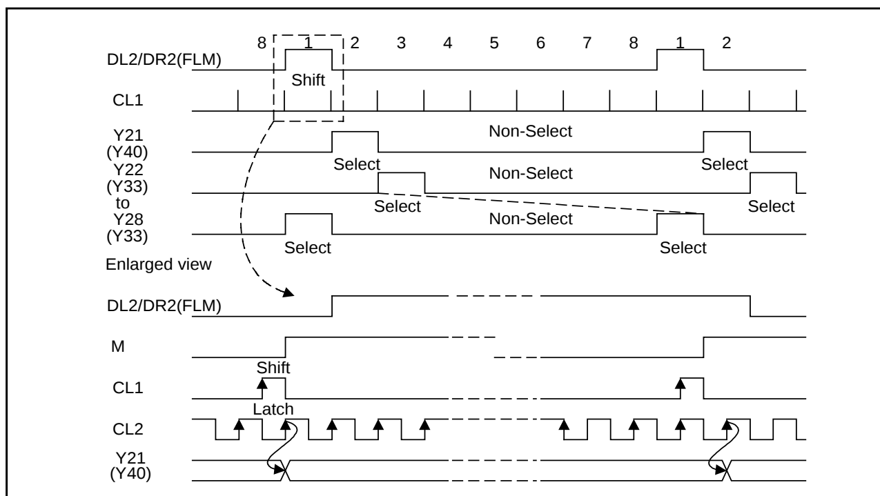
Common data waveforms ( A type waveforms of channel 2, 1/8 duty cycle )
