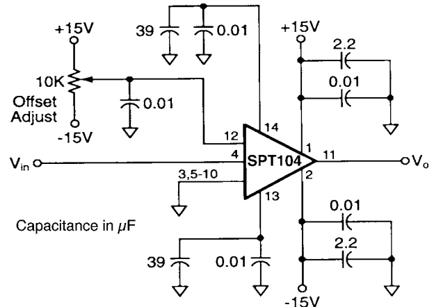
Figure 1: Basic Circuit
