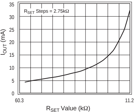
Figure 3: R_{SET} vs. I_{OUT}
