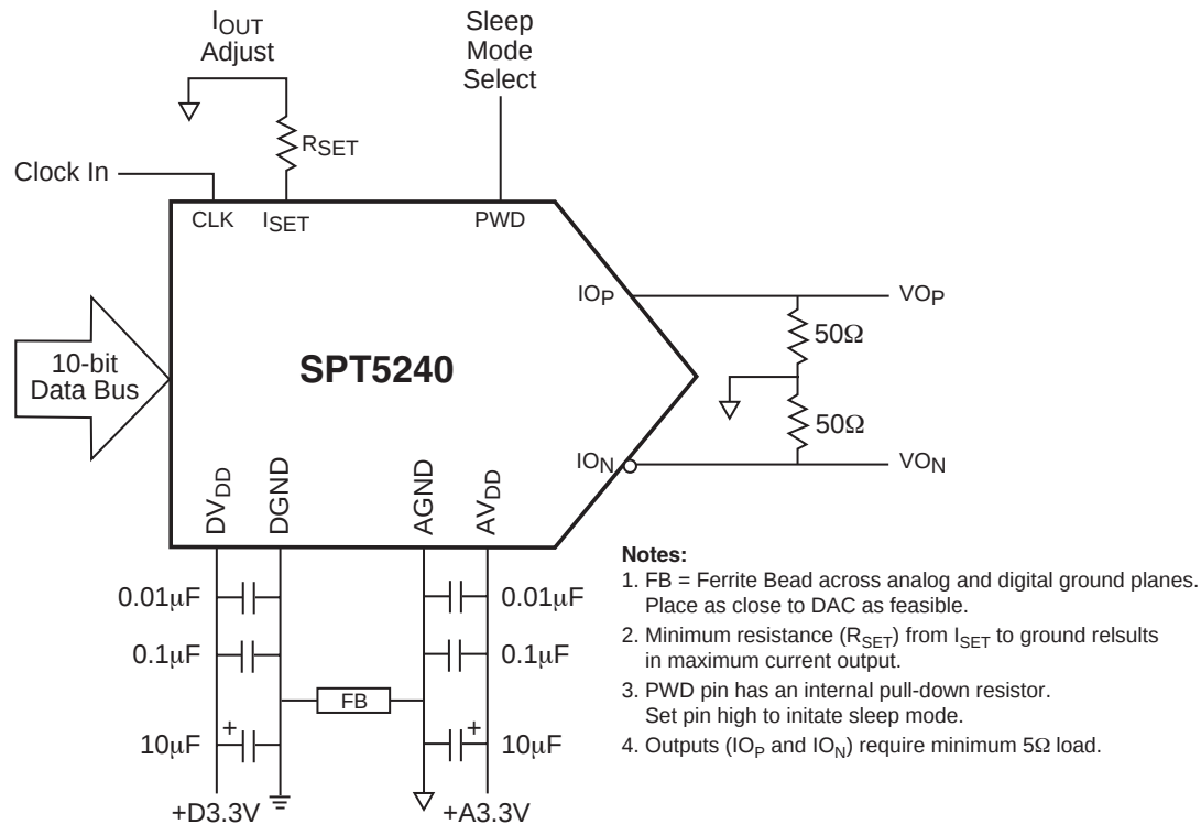
Figure 2: Typical Interface Circuit Diagram
