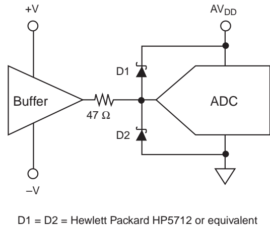
Figure 5 – Recommended Input Protection Circuit
