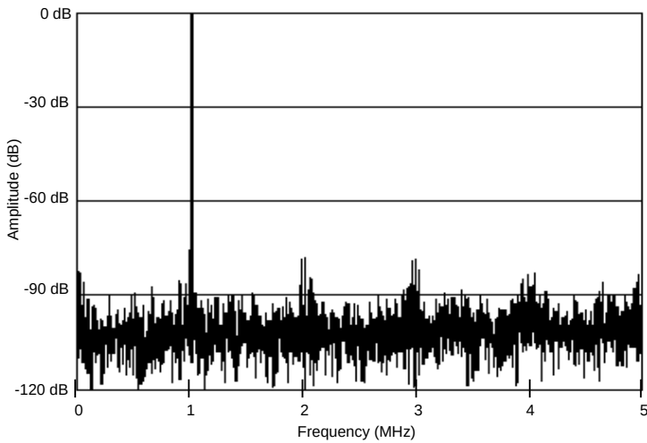
Spectral Response
