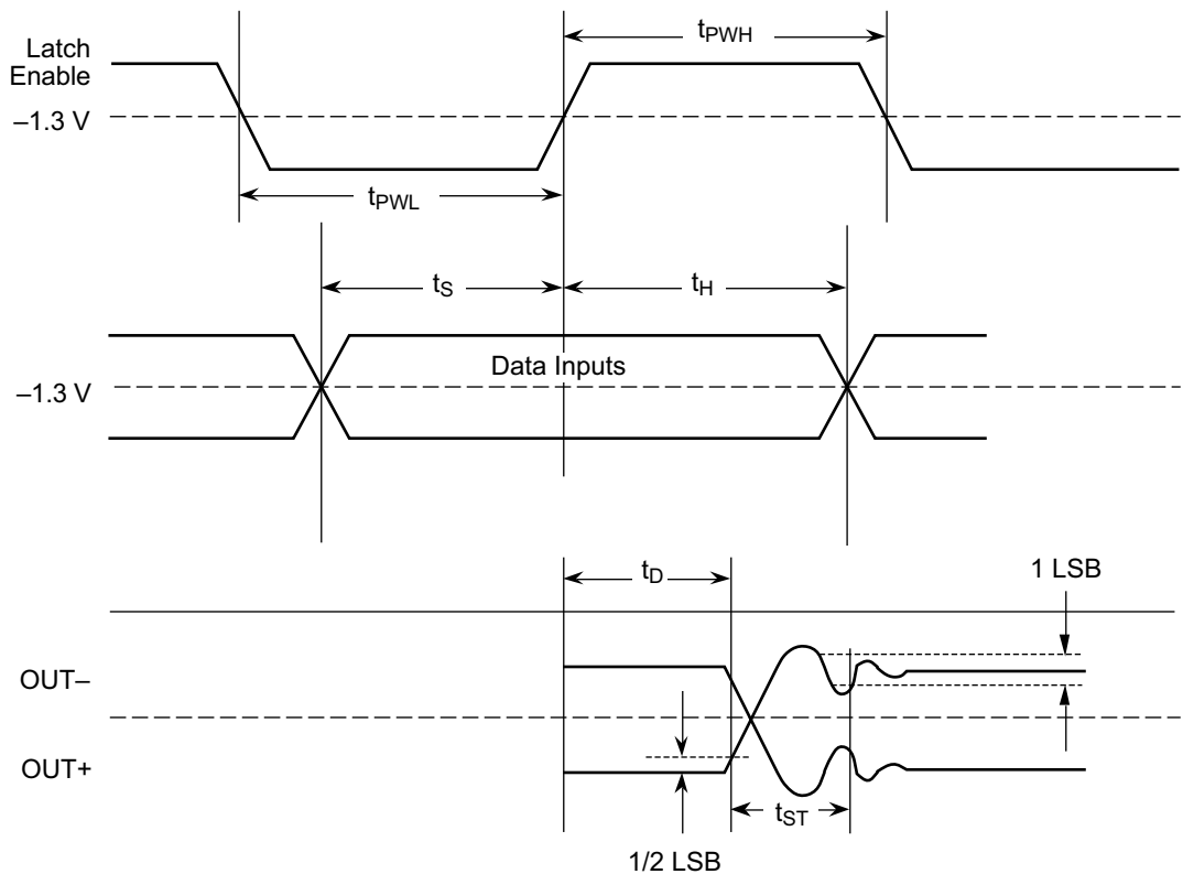
Figure 1 – Timing Diagram
