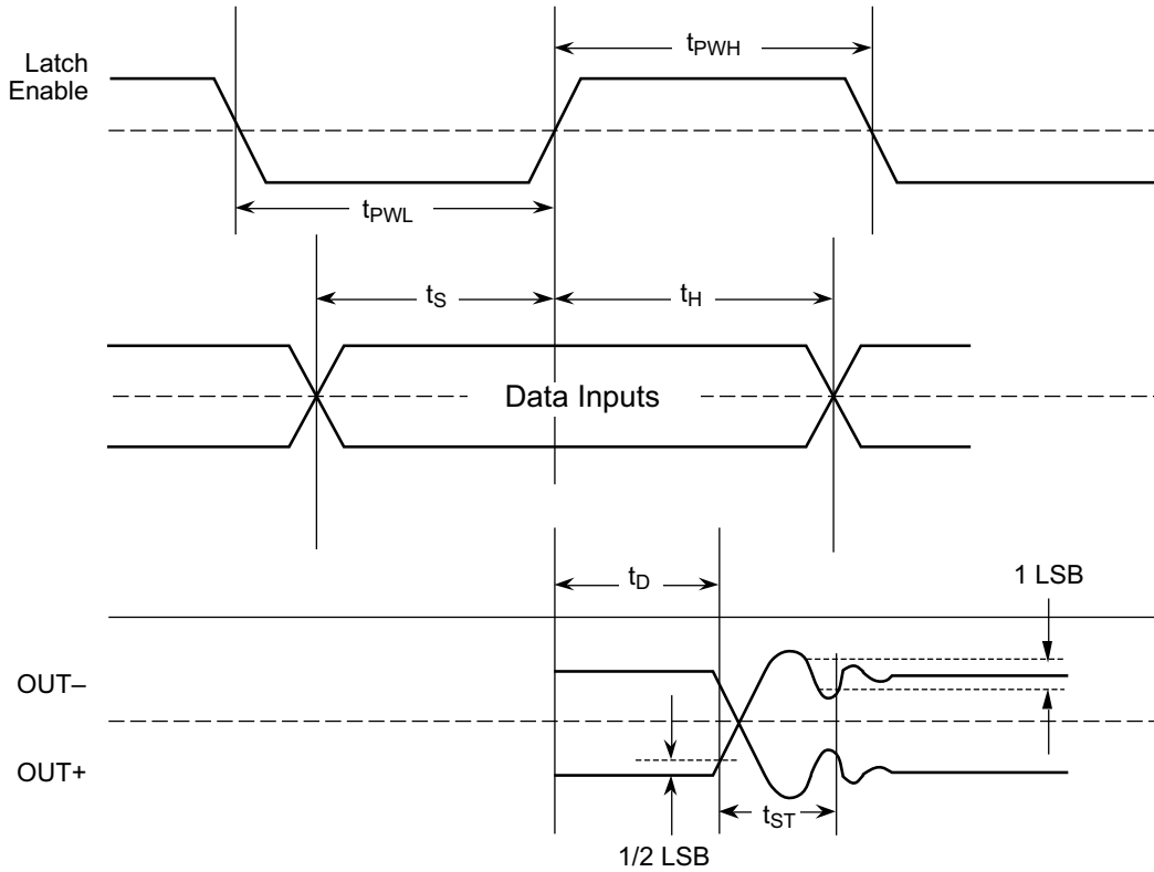
Figure 1 – Timing Diagram
