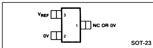
Fig. 1 Pin connections (top view)
