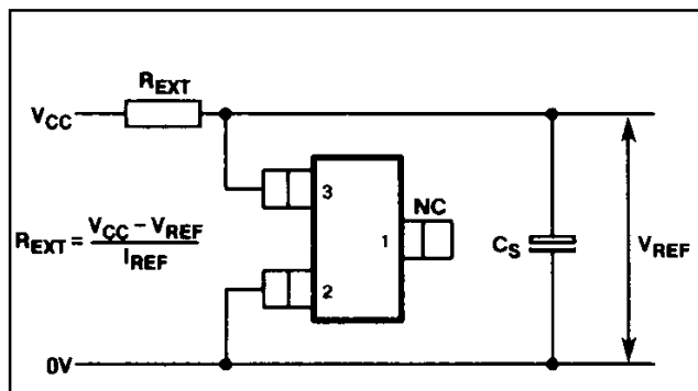
Fig.3 SR12D external connections.
