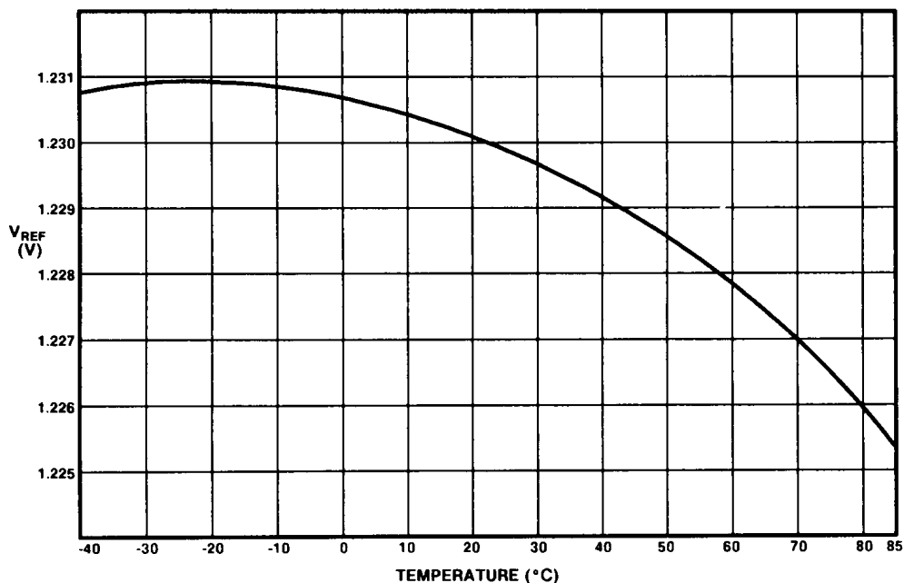
Fig.6 Typical temperature characteristic of SR12D at I_{REF} = 150 \mu A
