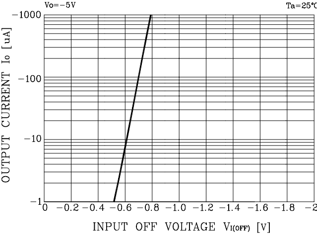
Fig. 2 I_o - V_{I(OFF)}
