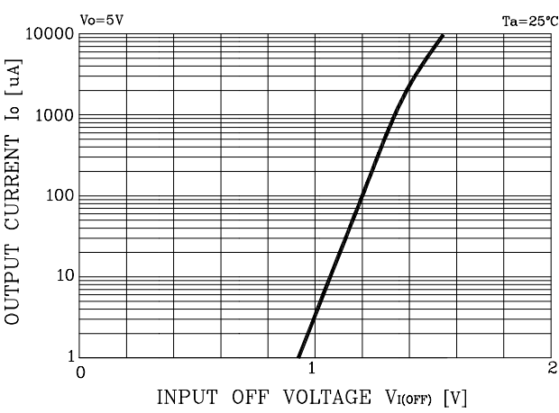
Fig. 2 I_O - V_{I(OFF)}
