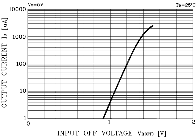
Fig. 2 I_o - V_{I(OFF)}
