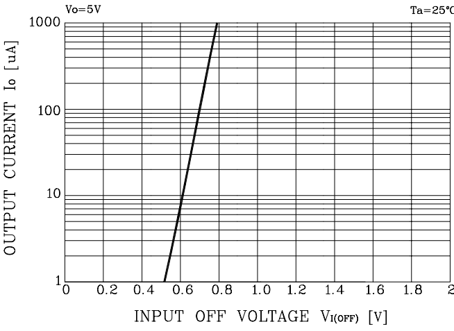
Fig. 2 I_O - V_{I(OFF)}
