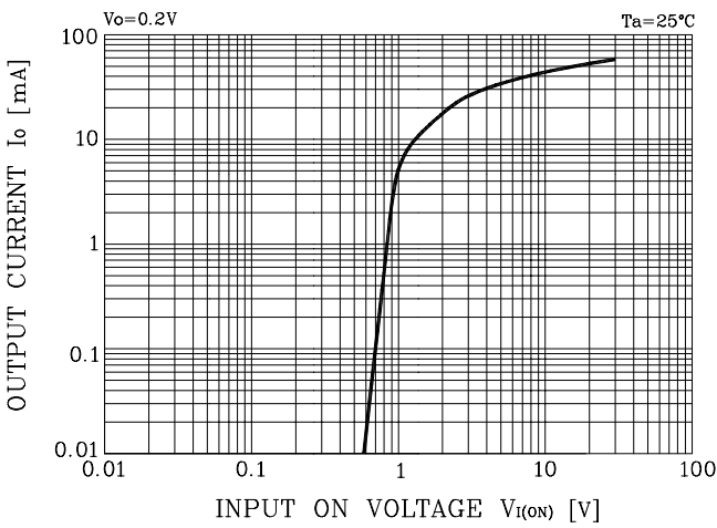
Fig. 1 I_O - V_{I(ON)}
