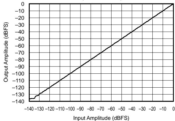
LINEARITY with f_{IN} = 200\text{Hz} (48kHz:44.1kHz)
