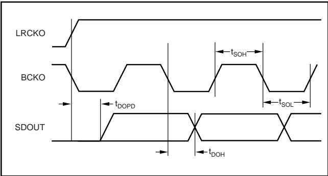
FIGURE 7. Output Port Timing.
