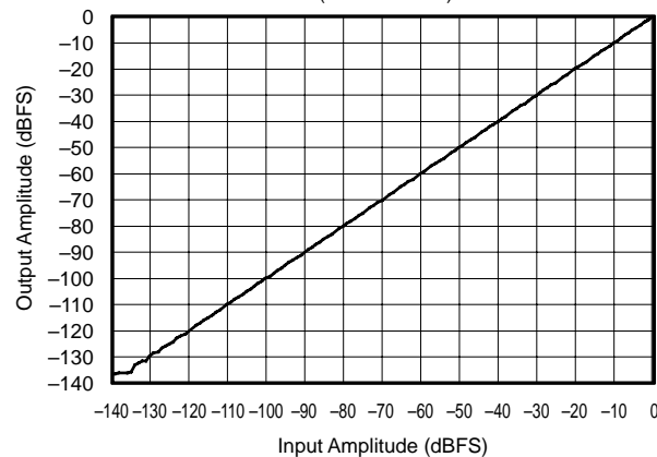
LINEARITY with f_{IN} = 200\text{Hz} (48kHz:96kHz)
