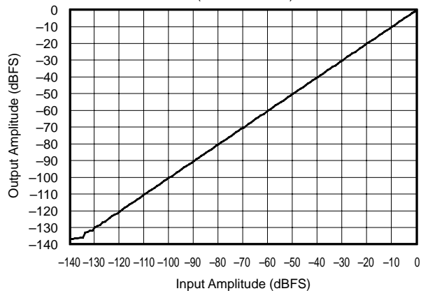
LINEARITY with f_{IN} = 200\text{Hz} (44.1kHz:48kHz)
