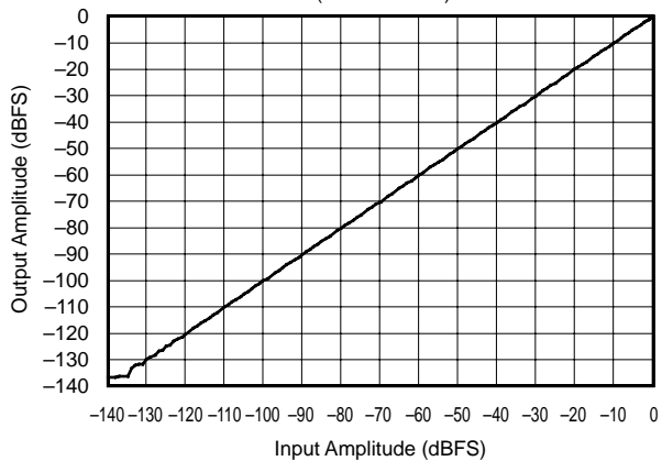
LINEARITY with f_{IN} = 200\text{Hz} (48kHz:48kHz)
