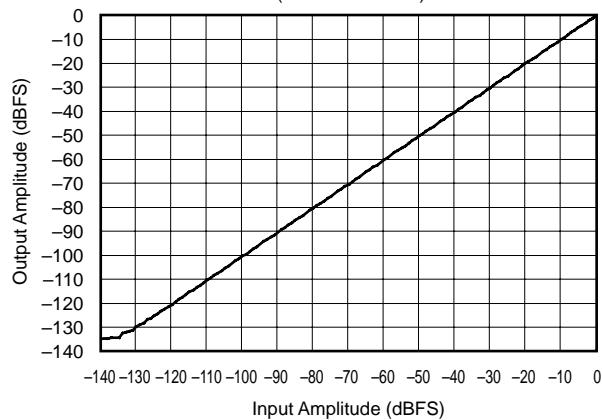
LINEARITY with f_{IN} = 200\text{Hz} (44.1kHz:192kHz)
