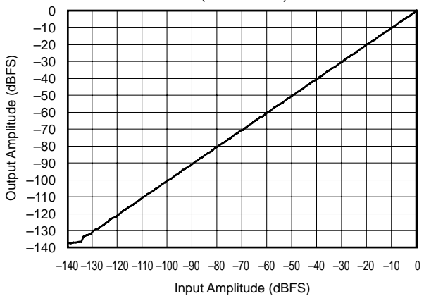
LINEARITY with f_{IN} = 200\text{Hz} (96kHz:48kHz)
