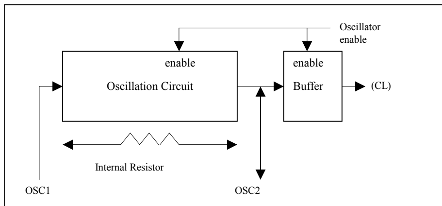
Figure 4 - Oscillator Circuitry
