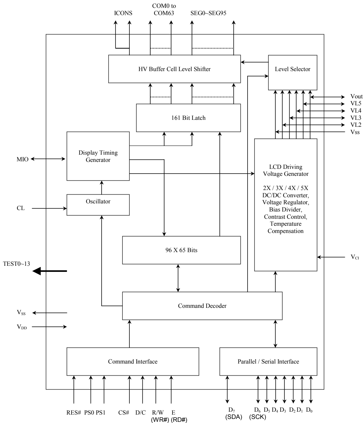
Figure 1 - Block Diagram
