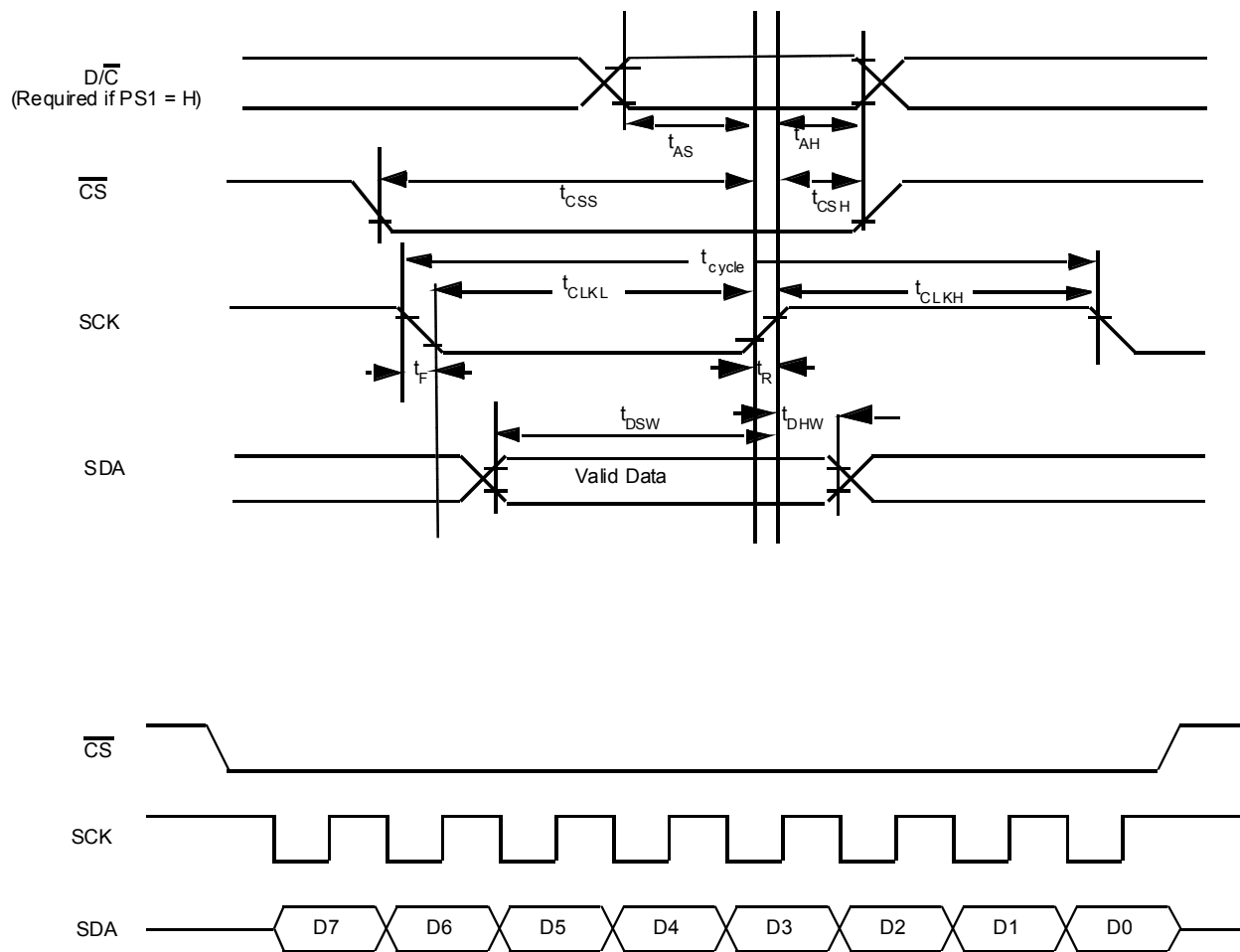
Figure 15 - Serial Timing Characteristics ( \text{PS0} = \text{L} )
