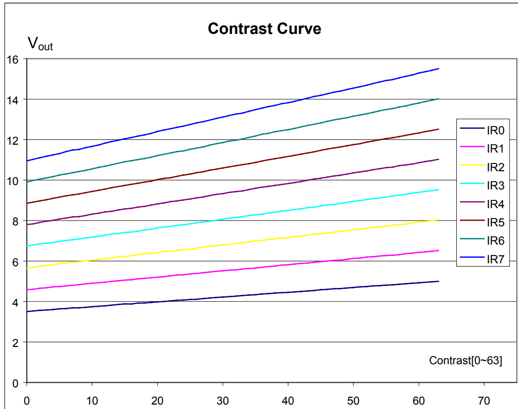
Figure 8 - Contrast Control Voltage Range Curve ( V_{DD}=2.775V ; V_{Cl}=3.5V ; TC=-0.05\%/^{\circ}C )
