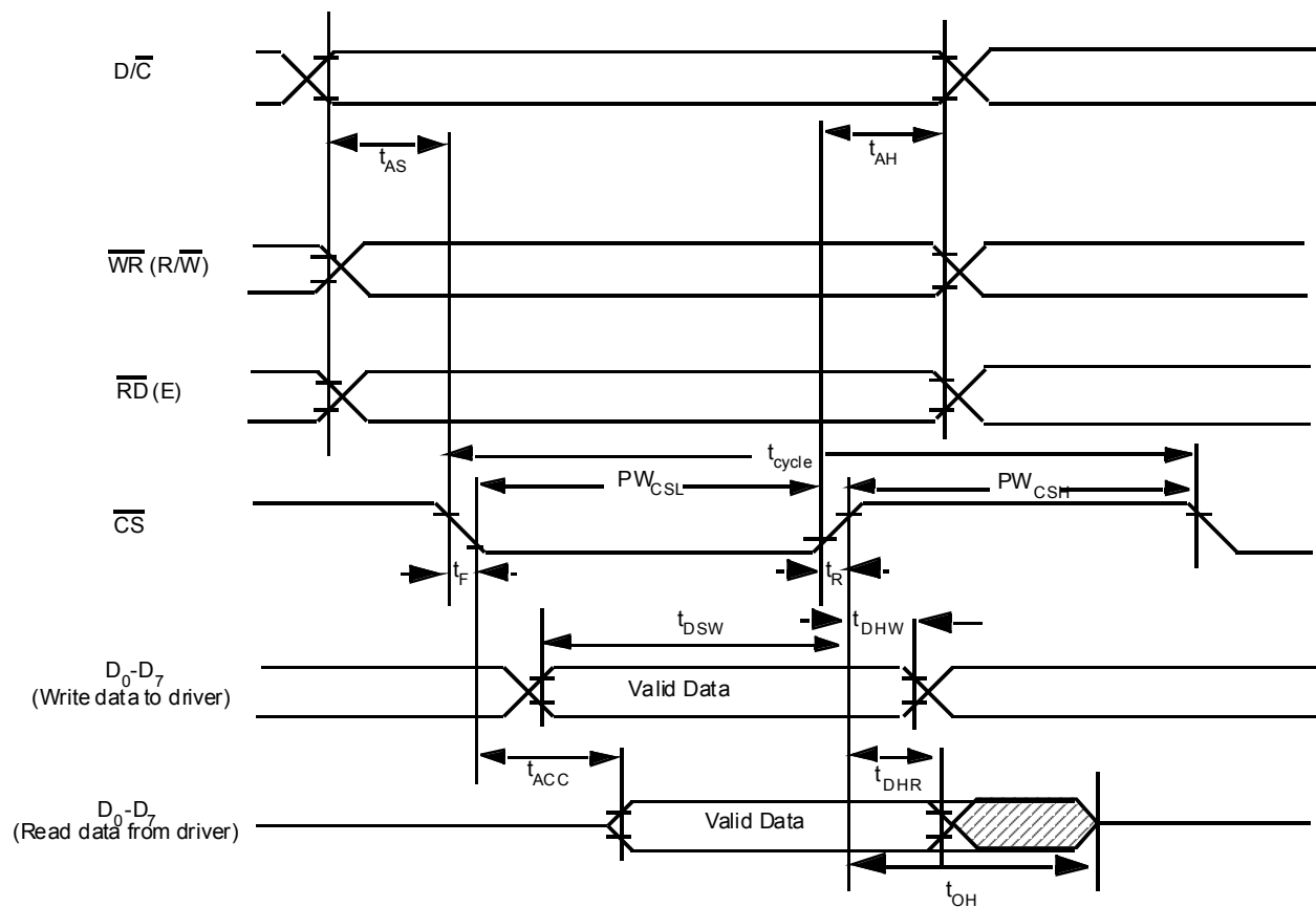
Figure 12 - Parallel 8080-series Interface Timing Characteristics (PS0 = H, PS1 = L)
