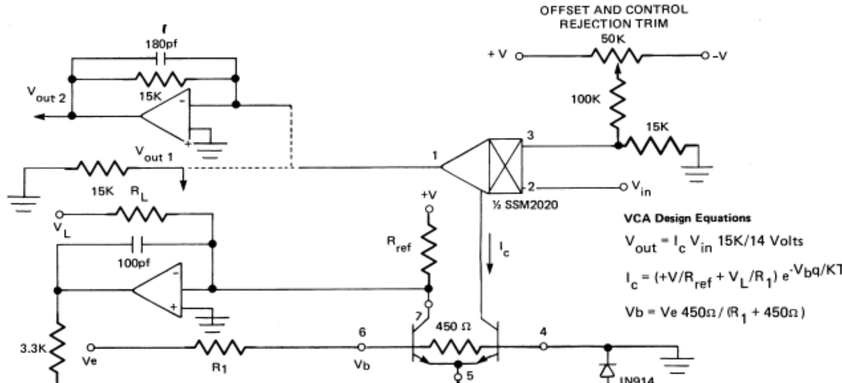
Voltage Controlled Filter (10,000 to 1 Sweep)
