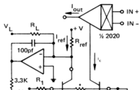
Basic Control Circuit
