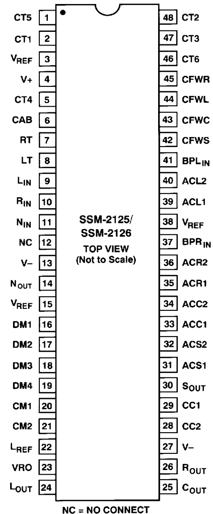
PIN CONNECTIONS
