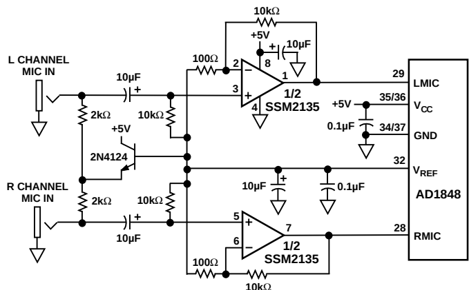
Figure 31. Low Noise Microphone Preamp for Multimedia Sound Codec
