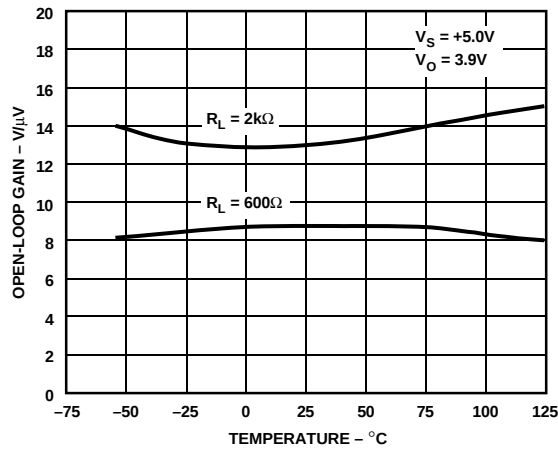
Figure 25. Open-Loop Gain vs. Temperature
