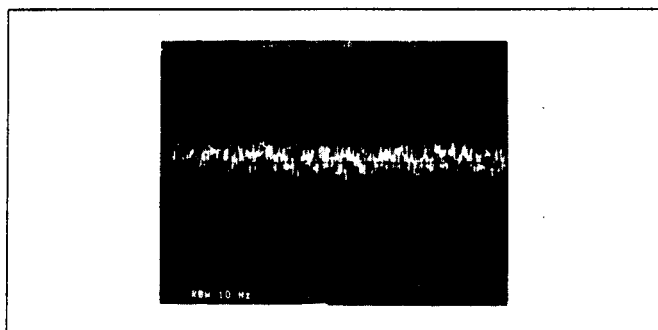
FIGURE 2: Spectrum Analyzer Display of Wideband Amplifier Noise Spectral Density. e_n \approx 1.7nV/\sqrt{Hz}
