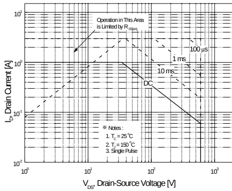
Figure 9-1. Maximum Safe Operating Area for SSP1N60B
