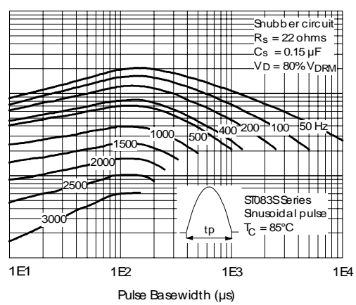
Fig. 11 - Frequency Characteristics
