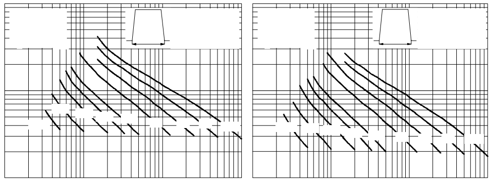
Fig. 12 - Frequency Characteristics
