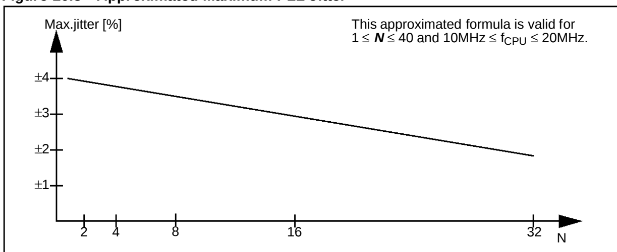
Figure 20.5 Approximated Maximum PLL Jitter
