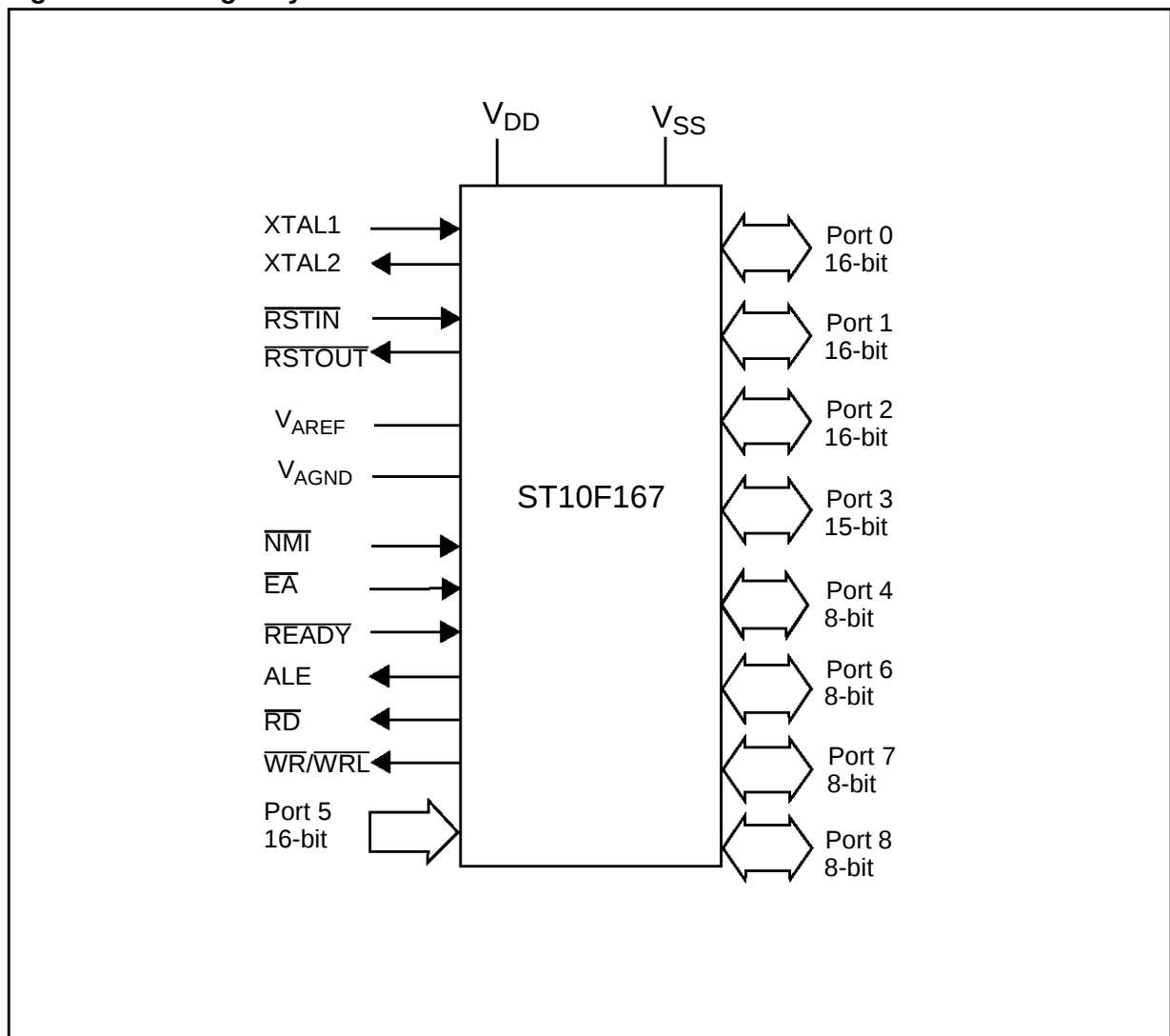
Figure 1.1 Logic Symbol
