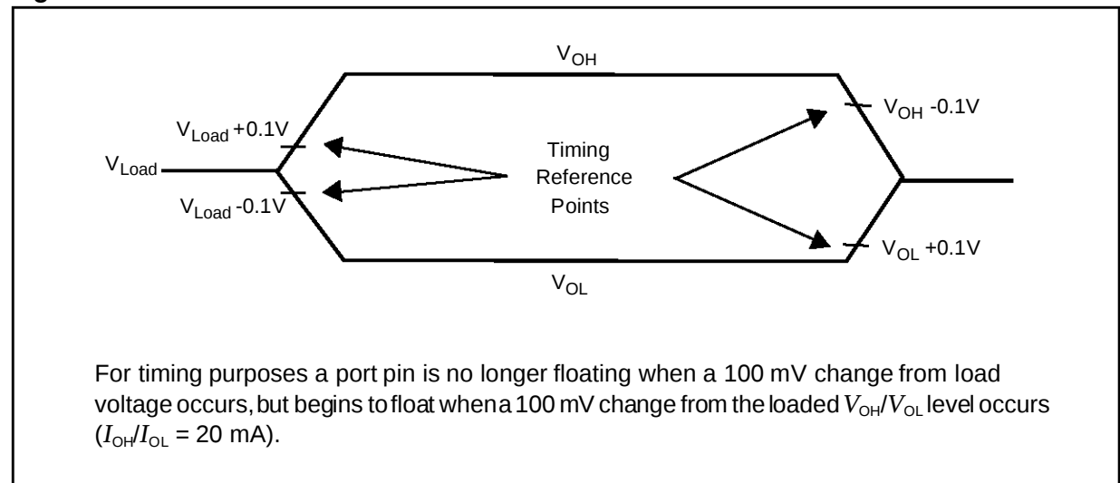
Figure 20.3 Float Waveforms
