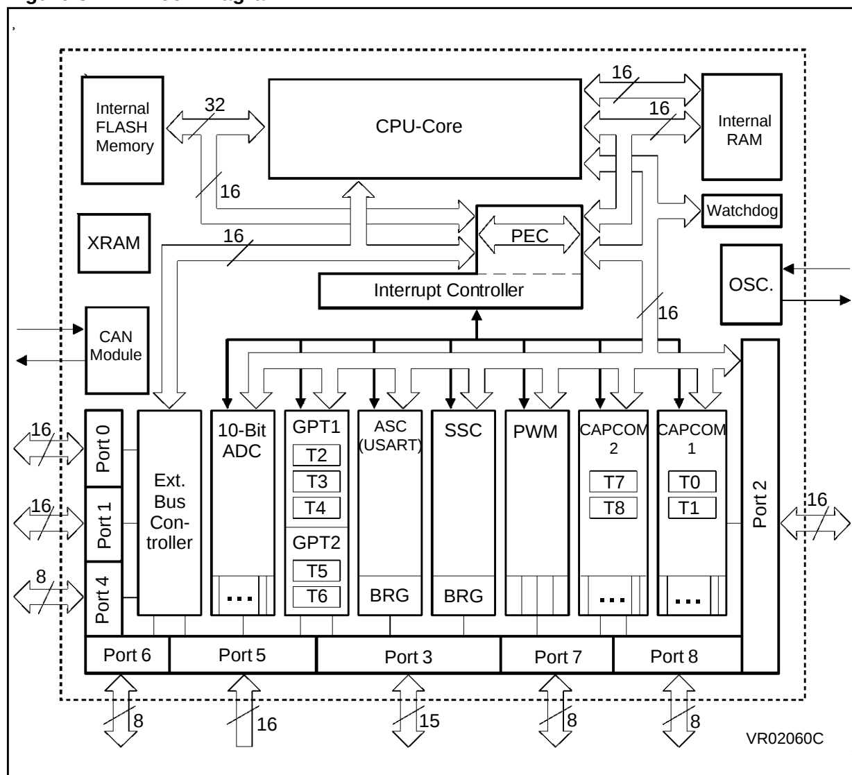
Figure 3.1 Block Diagram
