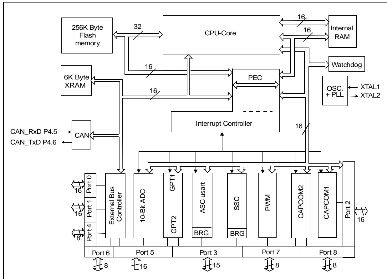
Figure 3 : Block Diagram
