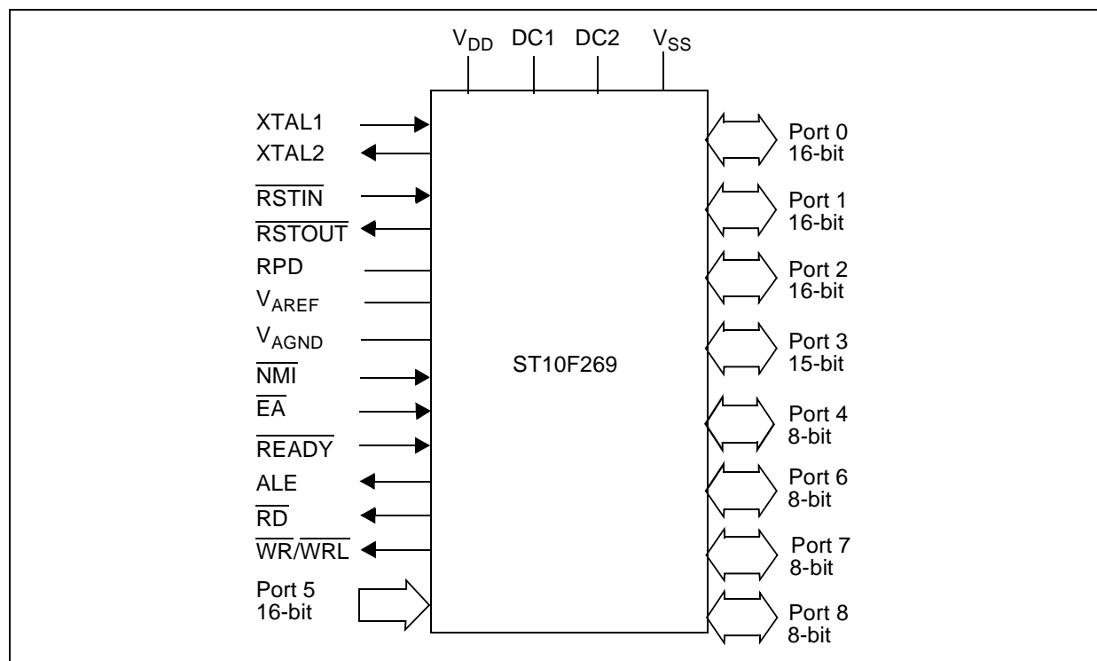
Figure 1 : Logic Symbol
