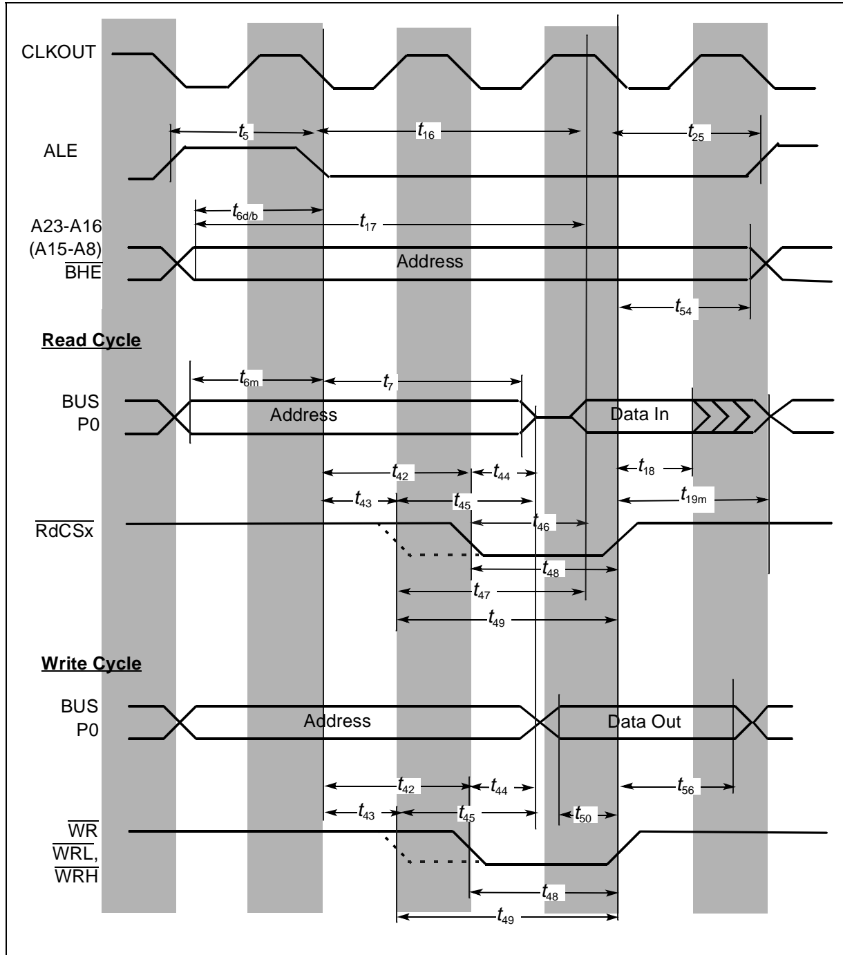
Figure 16 External memory cycle: multiplexed bus, with/without read/write delay, extended ale, read/write chip select
