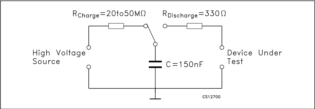
Figure 8: IEC 1000-4-2 Circuit
