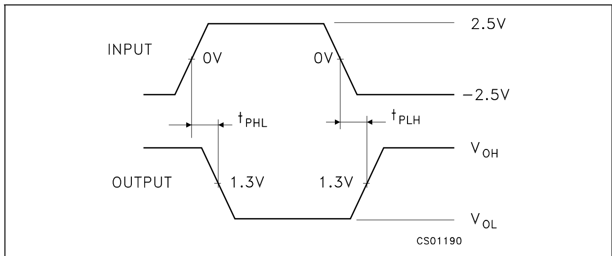
Figure 2 : Propagation Delays
