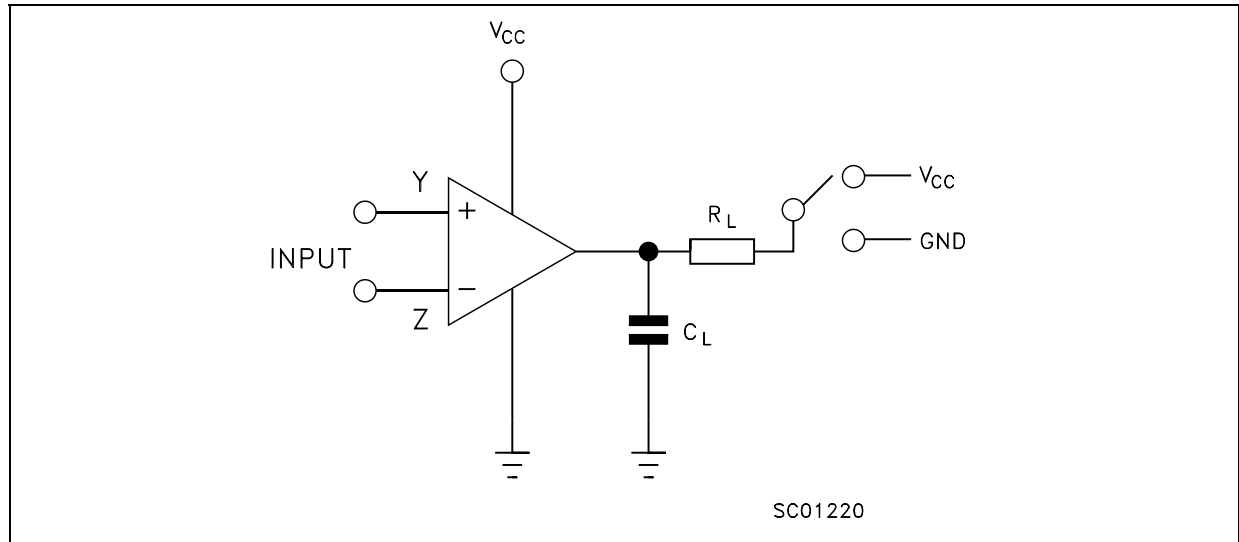
Figure 2 : Propagation Delays
