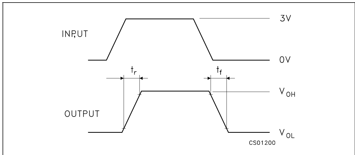
Figure 4 : Differential Rise and Fall Time
