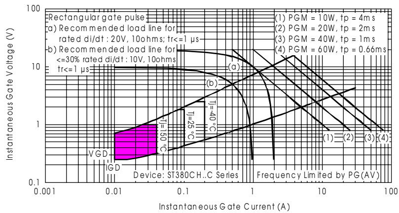
Fig. 11 - Gate Characteristics
