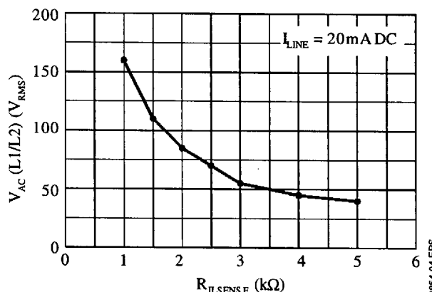
Figure 2 : Overvoltage Protection
