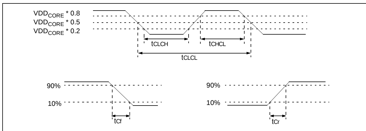
Figure 16: CLKIN timings
