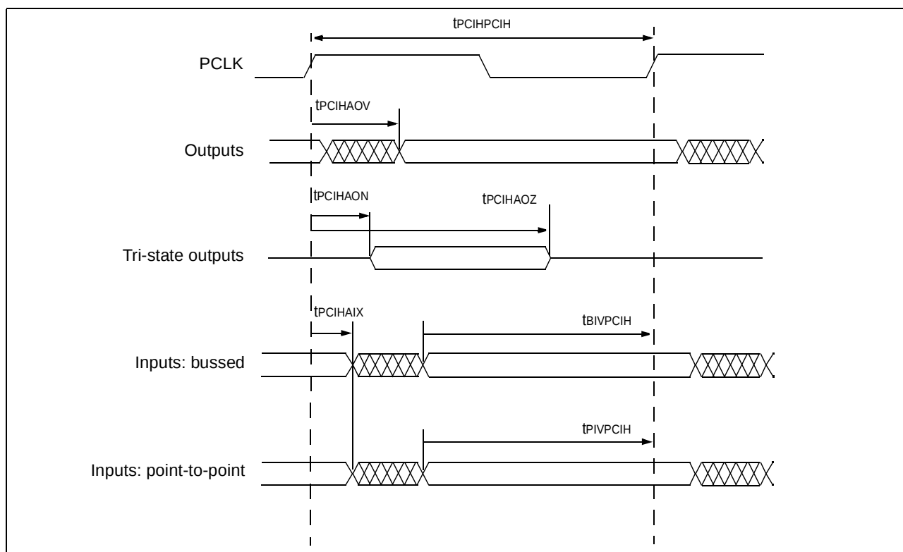
Figure 10: PCI timings
