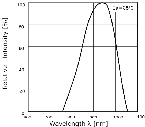
Fig. 5 Spectrum Sensitivity
