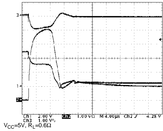
Figure 5 : Switching Waveforms,
