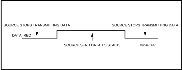
Figure 6. DATA_REQ control line
