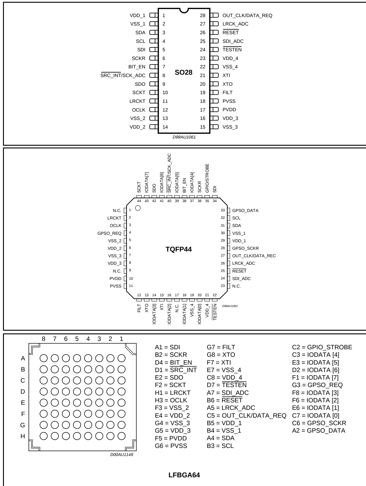
Figure 2. PIN CONNECTIONS
