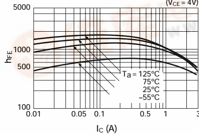
■ h FE — I C Temperature Characteristics (typ.) (V CE = 4V)
