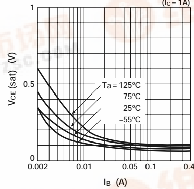
■ V CE(sat) — I B Temperature Characteristics (I C = 1A)
