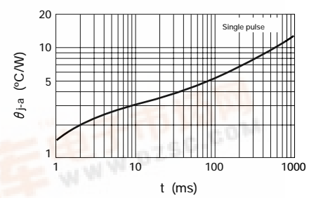
θ J-a — t Characteristics (Single pulse)
