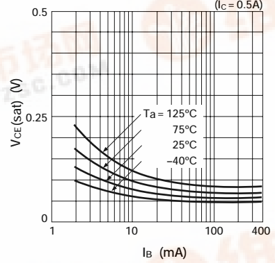
V CE(sat) — I B Temperature Characteristics (I C = 0.5A)
