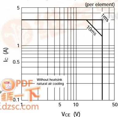
Safe Operating Area (single pulse) (per element)
