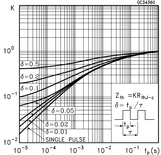
Thermal Impedance for IPAK
