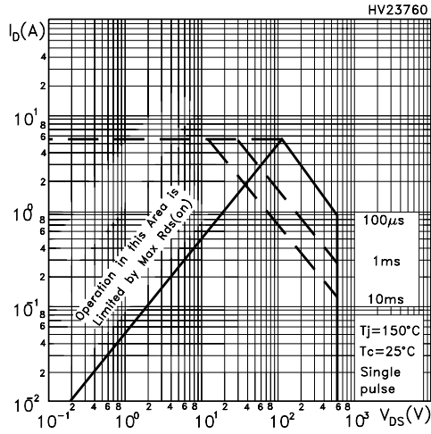
Figure 10: Output Characteristics
