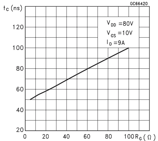
Figure 16. Cross-over Time
