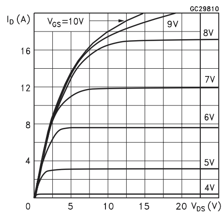
Figure 6. Output Characteristics
