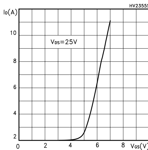
Figure 8: Transfer Characteristics
