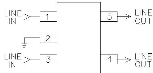
Figure 2 - STF701 Connection Diagram
