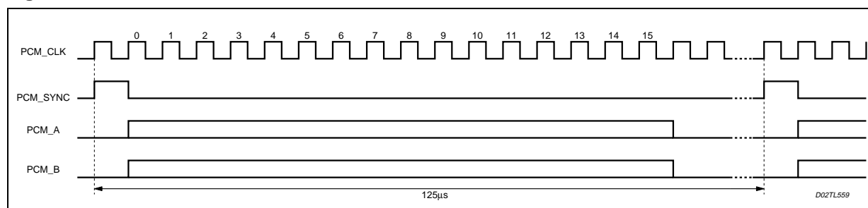
Figure 7. Linear Mode
