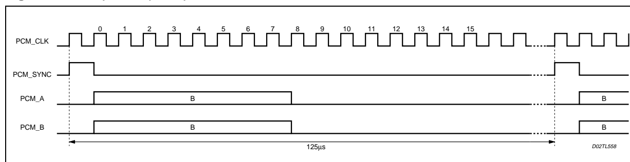
Figure 6. PCM (A-law, \mu -law) Standard Mode
