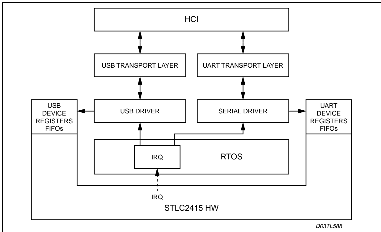
Figure 5. USB Interface
