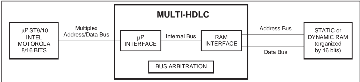
Figure 19 : Multi-HDLC connected to \mu P with non-multiplexed buses
