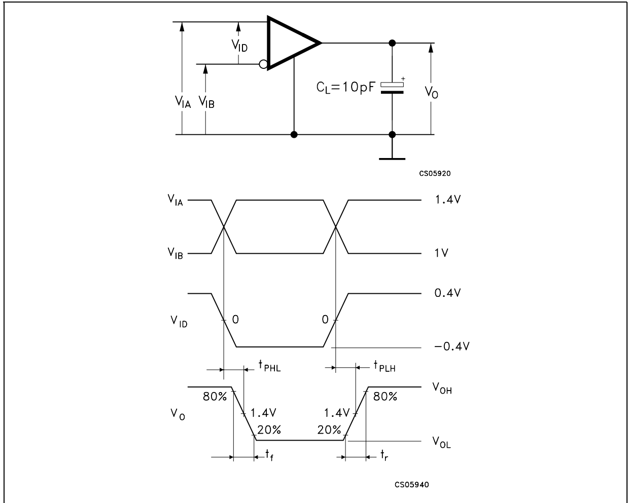
Figure 1 : Timing Test Circuit, Timing And Waveforms
