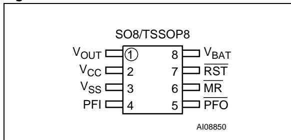
Figure 6. STM704/806 Connections
