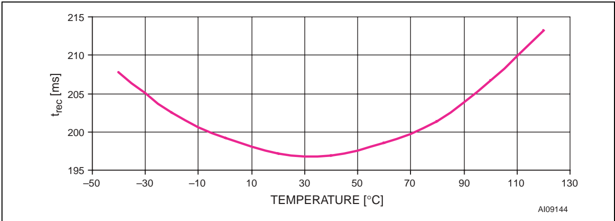
Figure 20. Power-up t_{rec} vs. Temperature
