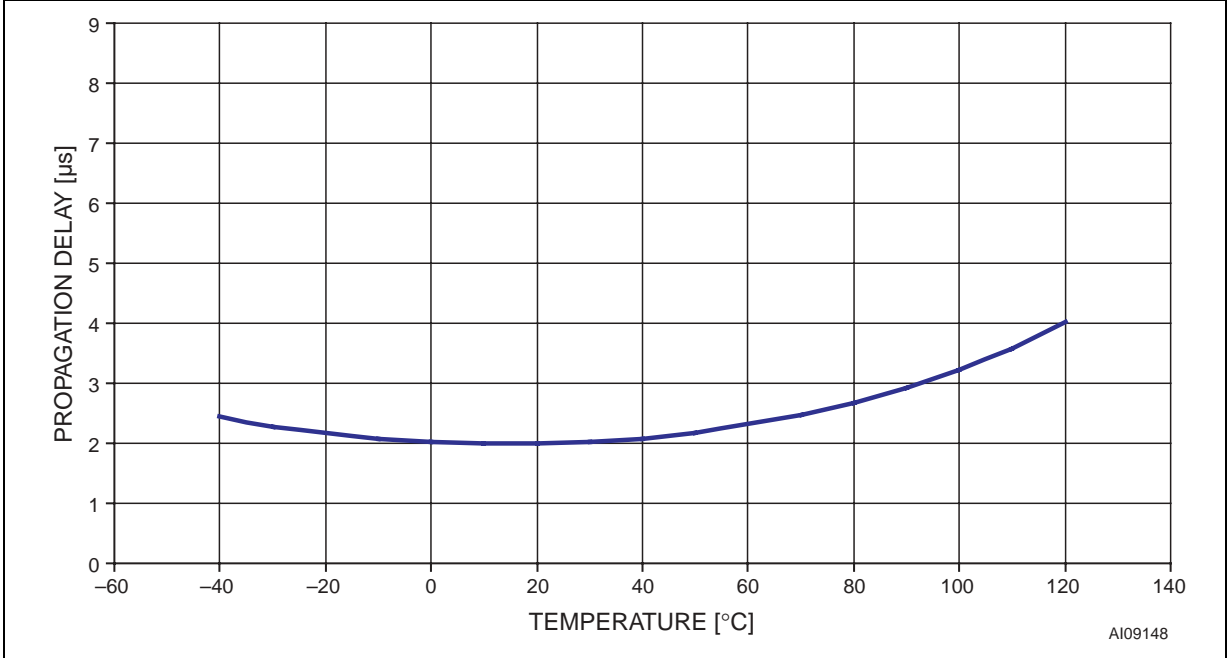
Figure 24. PFI to \overline{\text{PFO}} Propagation Delay vs. Temperature
