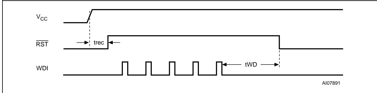
Figure 37. Watchdog Timing
