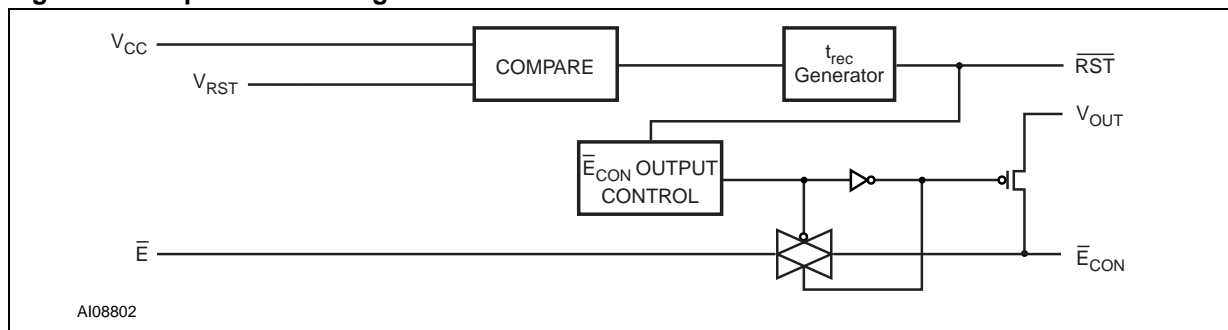
Figure 12. Chip-Enable Gating
