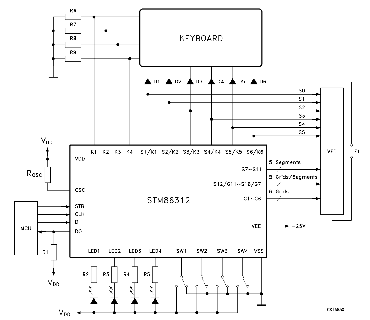
Figure 10: Application Circuit
