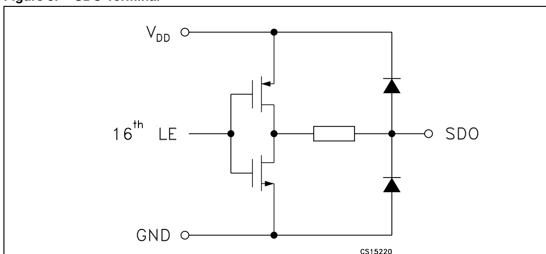
Figure 5. SDO Terminal
