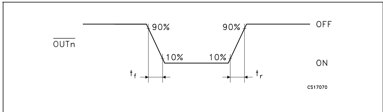
Figure 10: Outputs
