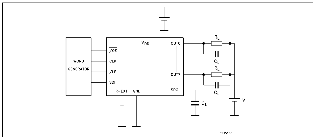
Figure 12: AC Characteristic
