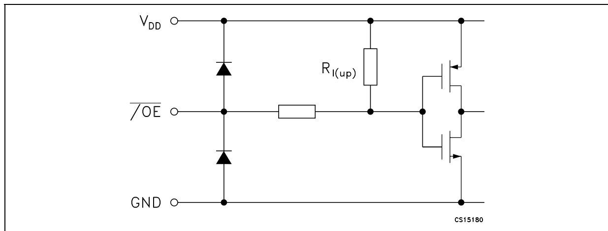
Figure 2: \overline{OE} Terminal
