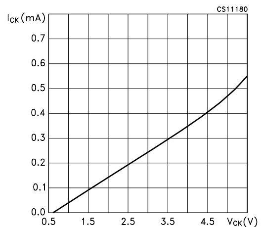
Figure 12 : Clock Leakage Current vs Clock Voltage
