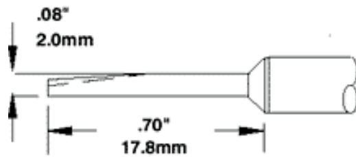
STTC-X83 Conical Grooved .08~ (2.0mm)
