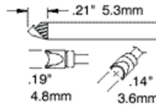
STTC-X97 Grooved Semi-Rigid Coax
