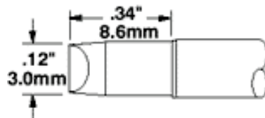
STTC-X03* Chisel 90° .12~ (3.0mm)
