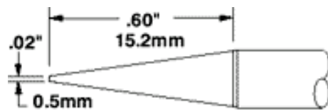
STTC-X43 Conical Sharp .02~ (0.5mm)
