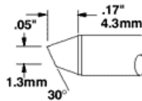
STTC-X15 Bevel 30° .05" (1.3mm)
