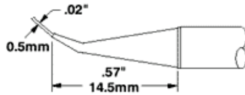
STTC-X44 Sharp Bent 30° .02~ (0.5mm)
