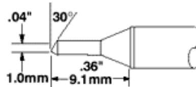
STTC-X24 Bevel 30° .04" (1.0mm)
