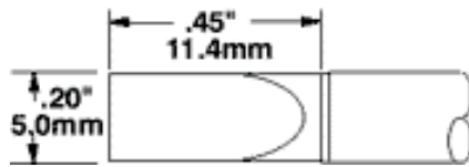
STTC-X65 Large Chisel .20~ (5.0mm)
