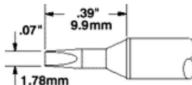
STTC-X37* Chisel 30° .07" (1.78mm)
