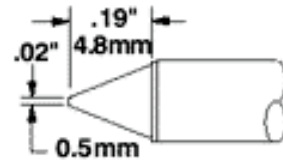
STTC-X16 Conical .02~ (0.5mm)
