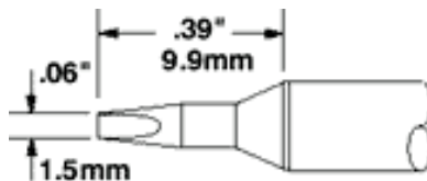
STTC-X38* Chisel 30° .06" (1.5mm)
