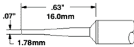
STTC-X42 Long Reach Chisel 60° .07" (1.78mm)
