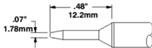
STTC-X02 Conical Sharp .07~ (1.78mm)
