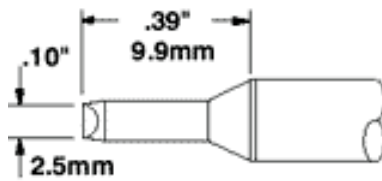
STTC-X33 Chisel 90° .10" (2.5mm)
