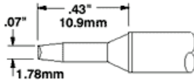
STTC-X04 Chisel 90° .07" (1.78mm)
