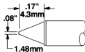
STTC-X12 Conical .08~ (2.03mm)
