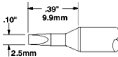
STTC-X36* Chisel 30° .10" (2.5mm)
