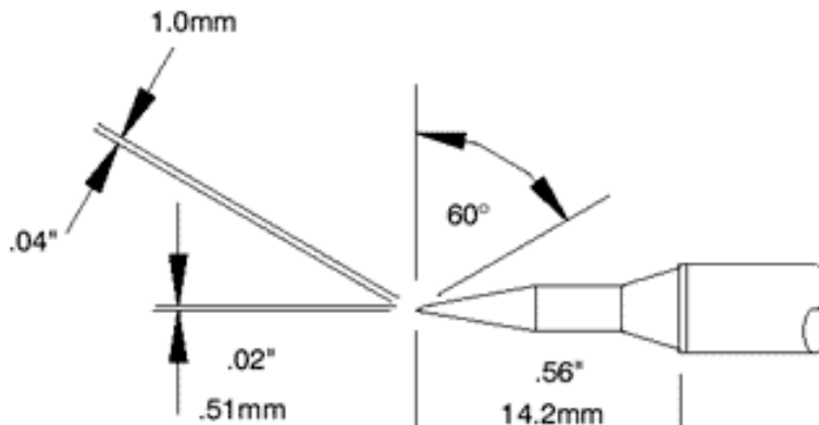
STTC-X46 Long Reach Bevel 60° .04" (1.0mm)
