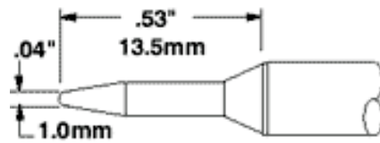
STTC-X01 Conical Sharp .04~ (1.0mm)
