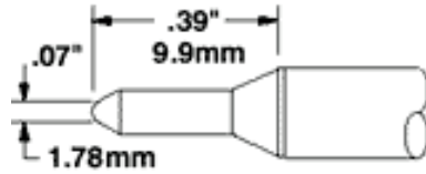
STTC-X32 Conical Sharp .07~ (1.78mm)
