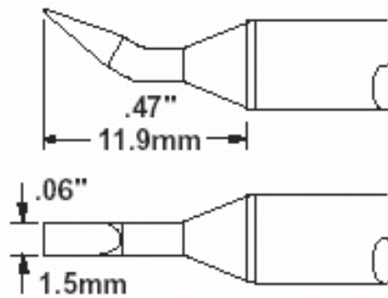
STTC-X99 Chisel Bent 30° .06" (1.5mm)
