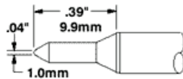
STTC-X31 Conical Sharp .04~ (1.0mm)
