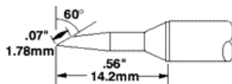
STTC-X47 Bevel 60° .07~ (1.78mm)
