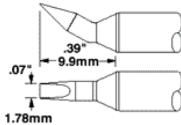
STTC-X98 Chisel Bent 30° .07" (1.78mm)
