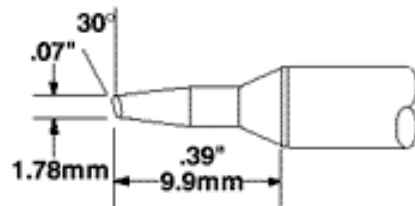
STTC-X35 Bevel 30° .07~ (1.78mm)
