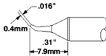
STTC-X26 Sharp Bent 30° .016~ (0.4mm)
