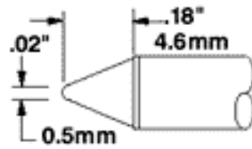
STTC-X11 Conical .02~ (0.5mm)
