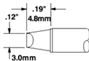
STTC-X13 Chisel 90° .12~ (3.0mm)
