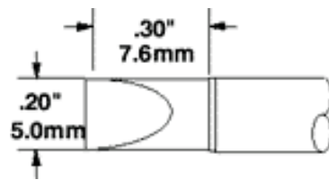
STTC-X17* Extra Large Chisel .20~(5.0mm)
