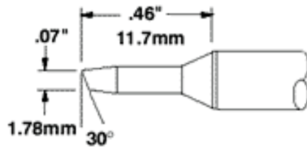
STTC-X05 Bevel 30° .07" (1.78mm)
